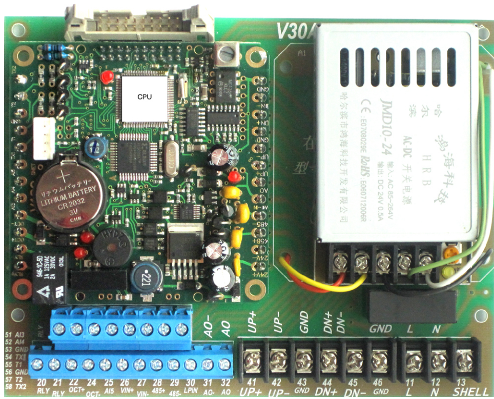
ground wire ( include upstream-ground wire and downstream ground wire ) 18 version mainboard
